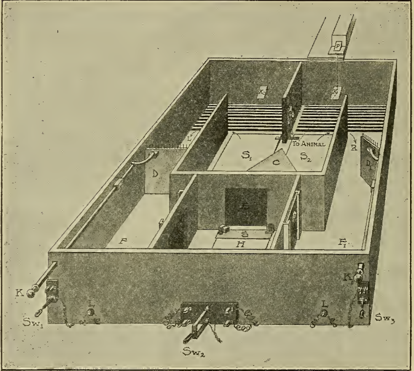
FIG. 1. CONTROL BOX
